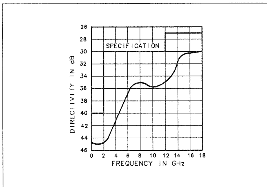
Figure 3. Directivity
